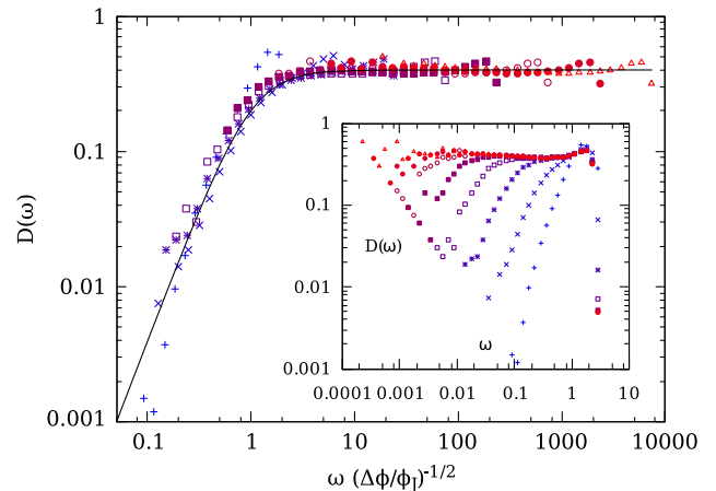
FIG. 1. DOS for a single configuration in d = 4 for N = 8192 with rescaled \omega . The collapsed data are fitted to Eq. (3) (solid line). Inset: DOS for \Delta\phi/\phi_J = 9.1 \times 10^{-8}, 9.2 \times 10^{-7}, 9.2 \times 10^{-6}, 9.2 \times 10^{-5}, 9.0 \times 10^{-4}, 8.7 \times 10^{-3}, 8.0 \times 10^{-2} , and 9.4 \times 10^{-1} , from left to right. Errors are smaller than the symbol size, except at very low \omega , where they are comparable to the data scatter.
