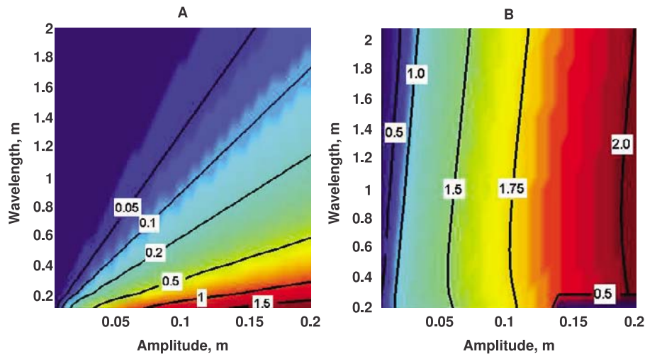
Figure 5. The increase in runoff initiation associated with the time to ponding and the storage time, both referenced against the time to ponding in the background case (see Table 1 for values). The proportional increases are rendered on a log scale to show their variation. (a) Time to ponding in the presence of microtopography relative to the background state and (b) Storage time associated with microtopography relative to the time to ponding. The runs were conducted with the usual reference properties and result in the change in total infiltration presented in Figure 4a.
