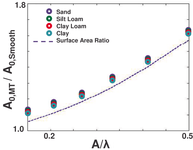
Figure 3. Effects of microtopography on infiltration dynamics based on a numerical solution to Richards' equation over a sinusoidal depression and for varying soil types. The effective sorptivity scales approximately 1:1 with the surface area ratio.
