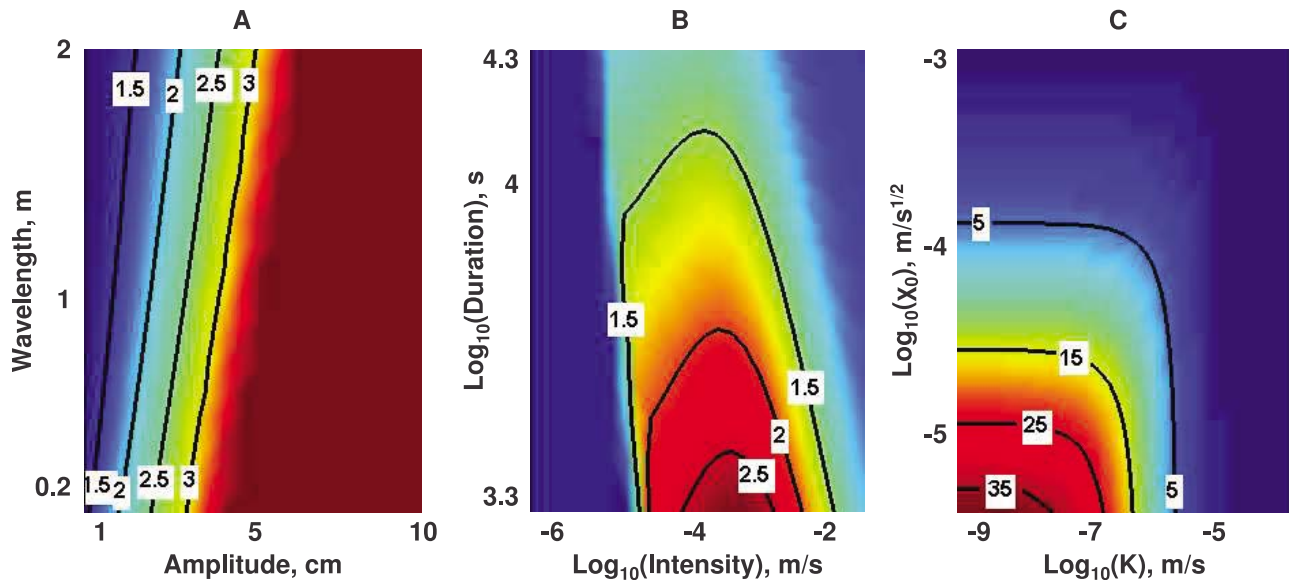
Figure 4. The proportional increase in infiltration per storm in the presence of microtopography ( A > 0 ) relative to the background state ( A = 0 ). Each plot represents variation in (a) microtopographic properties, (b) storm properties, and (c) soil properties about the background case (see Table 1).
