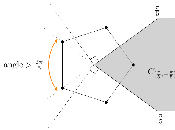
FIGURE 3. Example 2.1 in the case K = 5 .
