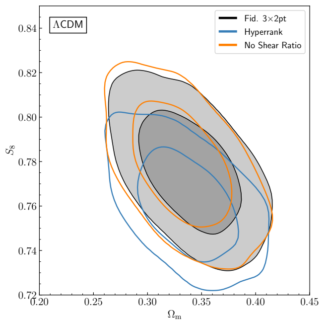
FIG. 25. A test of the impact of alternative redshift analysis choices on the inferred cosmology from 3\times 2 pt. We compare the fiducial 3\times 2 pt analysis (black) to an analysis where we marginalize over the ensemble of n(z) realizations directly via Hyperrank instead of their effective mean redshifts (blue) and to an analysis where we remove the shear-ratio data (orange).
