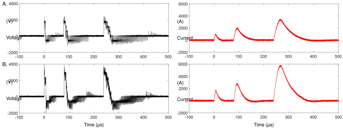
Figure 14. Sequence of monophasic pulses generated with various pulse durations and in two amplitudes. The approximately exponentially falling phase of the current in the second part of each pulse is generated through resistive damping in conventional monophasic TMS devices associated with the loss of the entire pulse energy. The pulse synthesizer, however, simulates only a resistor to the coil and extracts the energy back to the internal capacitors through proper control so that there is sufficient energy to generate such rapid sequences, which no conventional monophasic device can. Whereas we demonstrated the adjustment of the module voltages to tune the pulse strength in Figure 13, here the lower amplitude of the sequence in Panel A uses less module levels than Panel B to clarify the coarser quantization of this approach.
