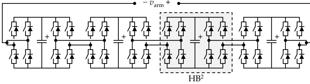
B. Example producing v_{arm} = 2
