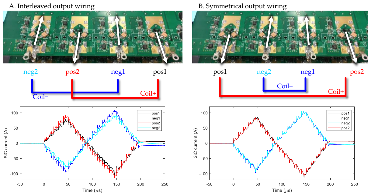
Figure 8. Two different assignments of four switching cells (discrete pair of high-side and low-side transistor) to two output bridges on one side of a module demonstrating the balance of the current among discrete parallel switching cells. Each switching cell contains discrete transistors (on the back, not visible), gate driver (black ICs between the golden islands), and first-level ceramic capacitance (yellow blocks in V configuration) to absorb the immediate energy demand and/or supply when the parasitic magnetic fields of the commutation current paths is discharged or charged.
