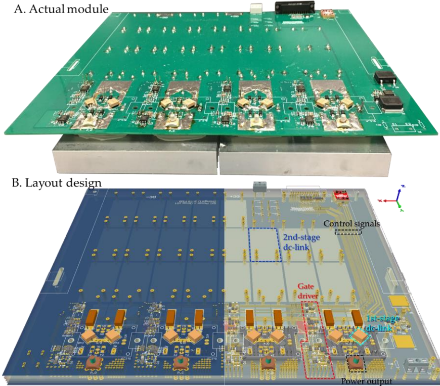
Figure 7. Circuit board layout (A. actual photo and B. design) with switching cells in the front and capacitance in the back. The transistors are on the bottom side, the driver and first-stage capacitance on the top.
