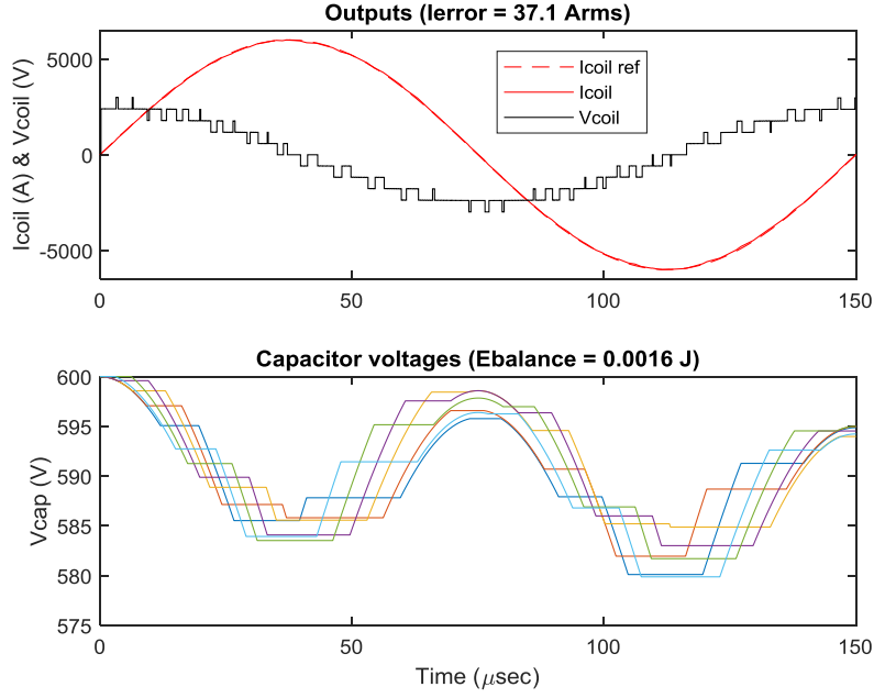
Figure 6. Simulation results using a reference that compensates the resistive voltage drop, module capacitor voltage variations, and the final module voltage spread.
