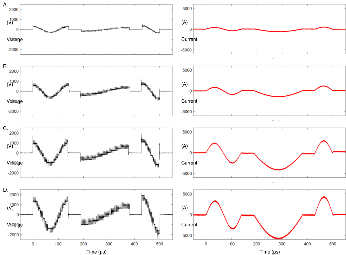
Figure 13. Recorded pulse train of typical conventional pulses (biphasic and two half-period pulses) with as little as 50 \mu\text{s} between two entirely different pulse shapes. The pulses have different energy content. Still, the device does not need any reconfiguration time or adjustment of charge to change the pulse duration, the pulse amplitude, or change the entire pulse shape. The panels from A to D show the same pulse sequence with increasing pulse amplitude. The recordings demonstrate both ways how the pulse synthesizer can adjust the pulse amplitude: Within a sequence, the circuit uses fewer steps for the lower-amplitude sections and pulses such as the long half-period pulse in the center. From pulse train to pulse train, the circuit increases the amplitude through increasing the module voltage step size.
