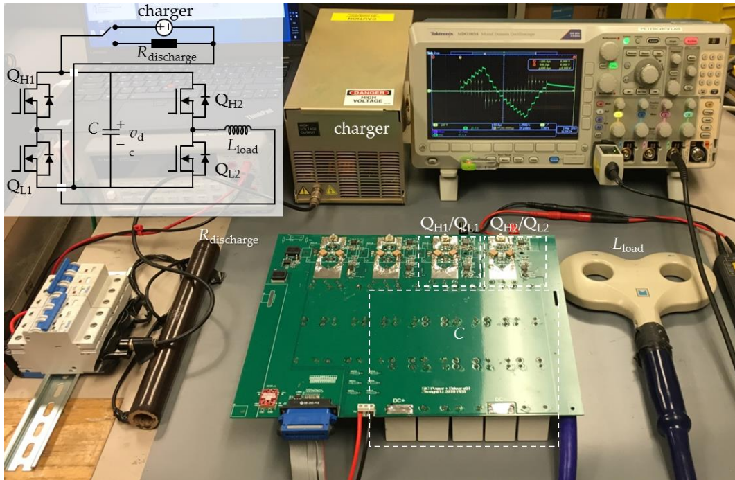
Figure 9. Double-pulse setup.
