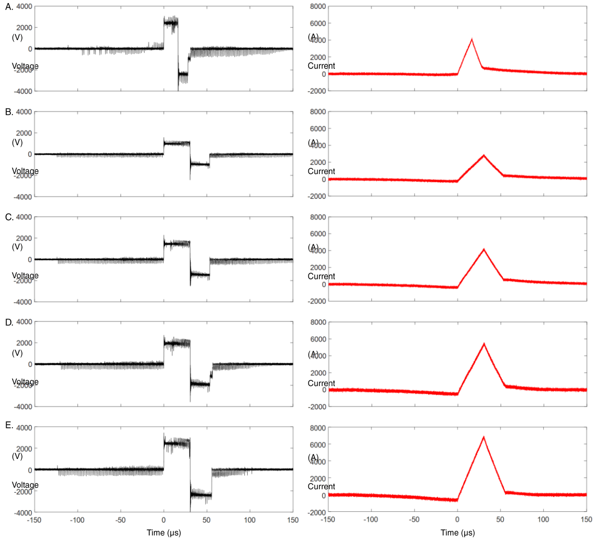
Figure 18. Pulse shapes optimized for minimum coil heating with different pulse duration (A and B) and various pulse amplitudes for the longer duration (B – E). Before the actual pulse, the device brings the current baseline slowly to a negative offset, from which the current can ramp up with a longer rising edge without reaching large currents. This pre-phase is generated through subtle control of the voltage in the approximately 120 \mu\text{s} introducing the pulse.
