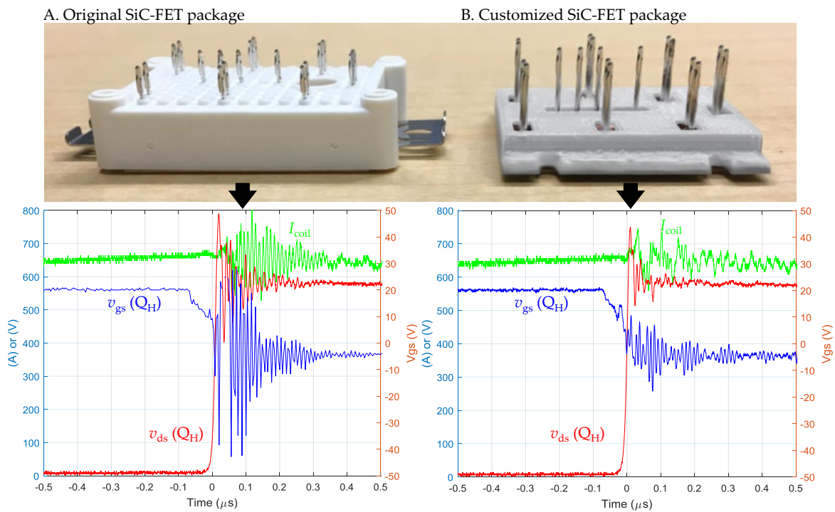
Figure 10. Example for one of four commutation conditions for A the original FF11 transistor bridge in the optimized layout and B with an optimized package for lower stray inductance. In the measurements, one transistor module is singled out.
