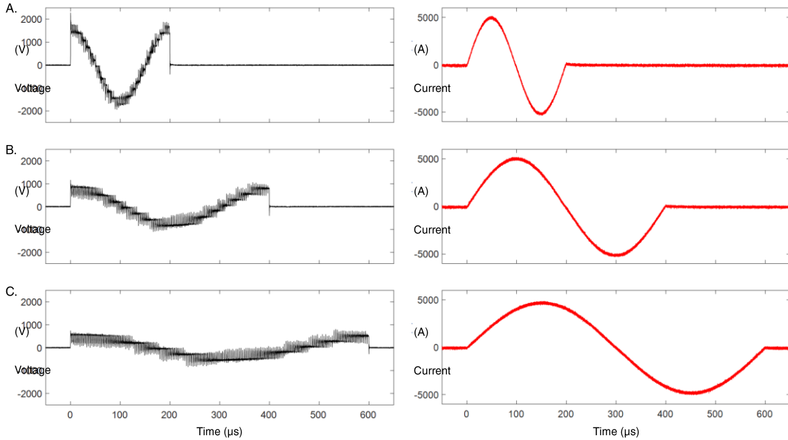
Figure 12. Recordings of biphasic pulses with sinusoidal voltage as well as electric field shape and sinusoidal current shape. The pulse shape including its duration is purely software-generated (A 200 \mu s, B 400 \mu s, C 600 \mu s).
