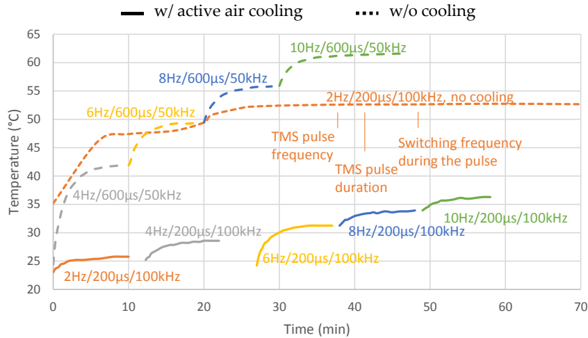
Figure 11. Temperature development of the SiC transistors under stress testing with sinusoidal current (700 A peak) per discrete transistor (enabling 8,400 A for a module with 12 transistors in our system) and transistor switching rates up to 100 kHz. Dashed lines were performed without any additional cooling in a closed 19” cabinet, solid lines included active air convection, demonstrating headroom. The temperature development and the steady-state temperatures show a widely linear relationship with the load as expected. The naming convention is pulse rate (Hz)/pulse duration /switching rate during the pulses.
