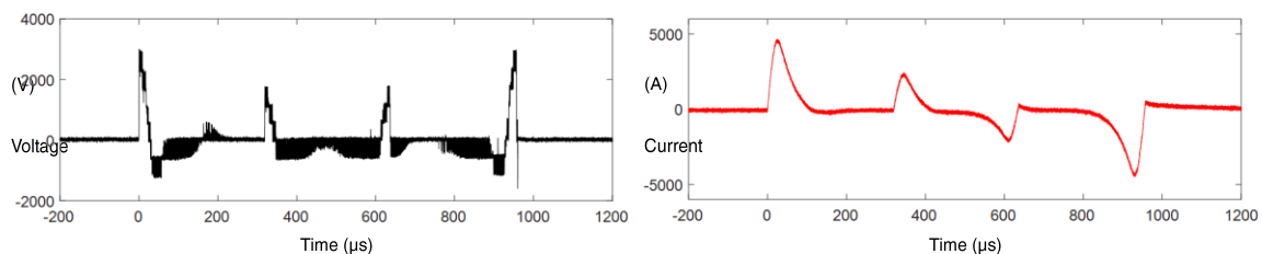
Figure 15. Burst of various monophasic pulses with different amplitude and time direction. To demonstrate the flexibility and ability to generate practically any pulse shape, the burst does not only change the amplitude but inverts the time direction for the third and fourth pulse so that the voltage is mirrored and the current additionally inverted.
