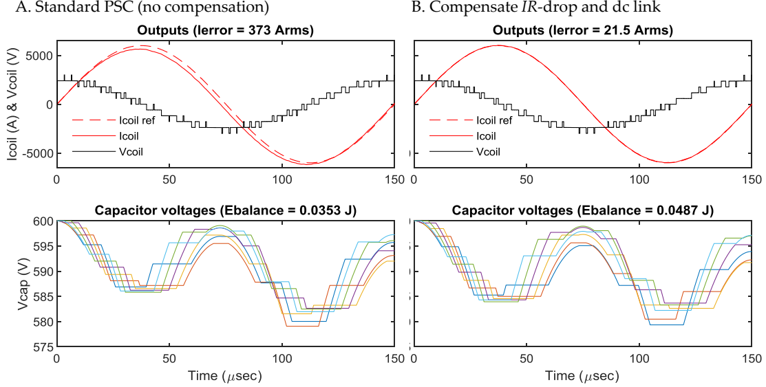
Figure 5. Simulation results (A) without compensation and (B) with a reference compensating resistive voltage drop and module capacitor voltage variations. The model does not use the parallel mode but only series and bypass to demonstrate how the capacitors drift apart. Parallelization clears such voltage differences.
