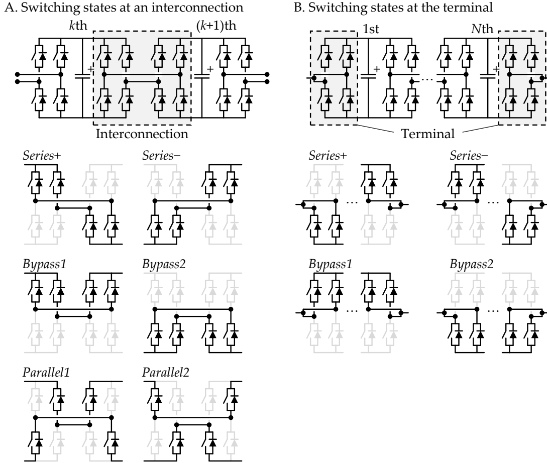
Figure 3. Switch states of an interconnection A between two modules or B the outmost modules connecting to the coil. The states influence how the capacitors of the modules are electrically connected relative to their neighbors. Two-bridge modules can generate only series and bypass states, four-bridge modules additionally parallel circuit configurations between modules. Series states increase the voltage in positive or negative direction. Parallel modes distribute the current load and balance charge across the capacitors. With fast transistors, the transition from one state to another can occur on the order of 100 ns and several hundred times per millisecond.
