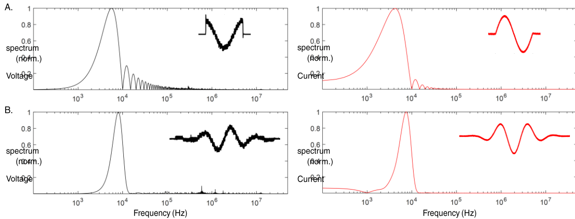
Figure 19. Unfiltered voltage and current spectra of (A) a biphasic pulse, which may mostly be dominated by an oscillation with one dominant frequency but inherently displays a wide spectrum to its brevity (frequency–time uncertainty principle), and (B) a polyphasic pulse with more periods and Gaussian envelope for a sharper spectrum of the intended pulse. With a careful look, one can see the small residual distortion due to both measurement noise and technical quantization emerging at the right side of the voltage spectrum, in the high-frequency range. The inset in each panel shows the corresponding time course of the voltage or current.
