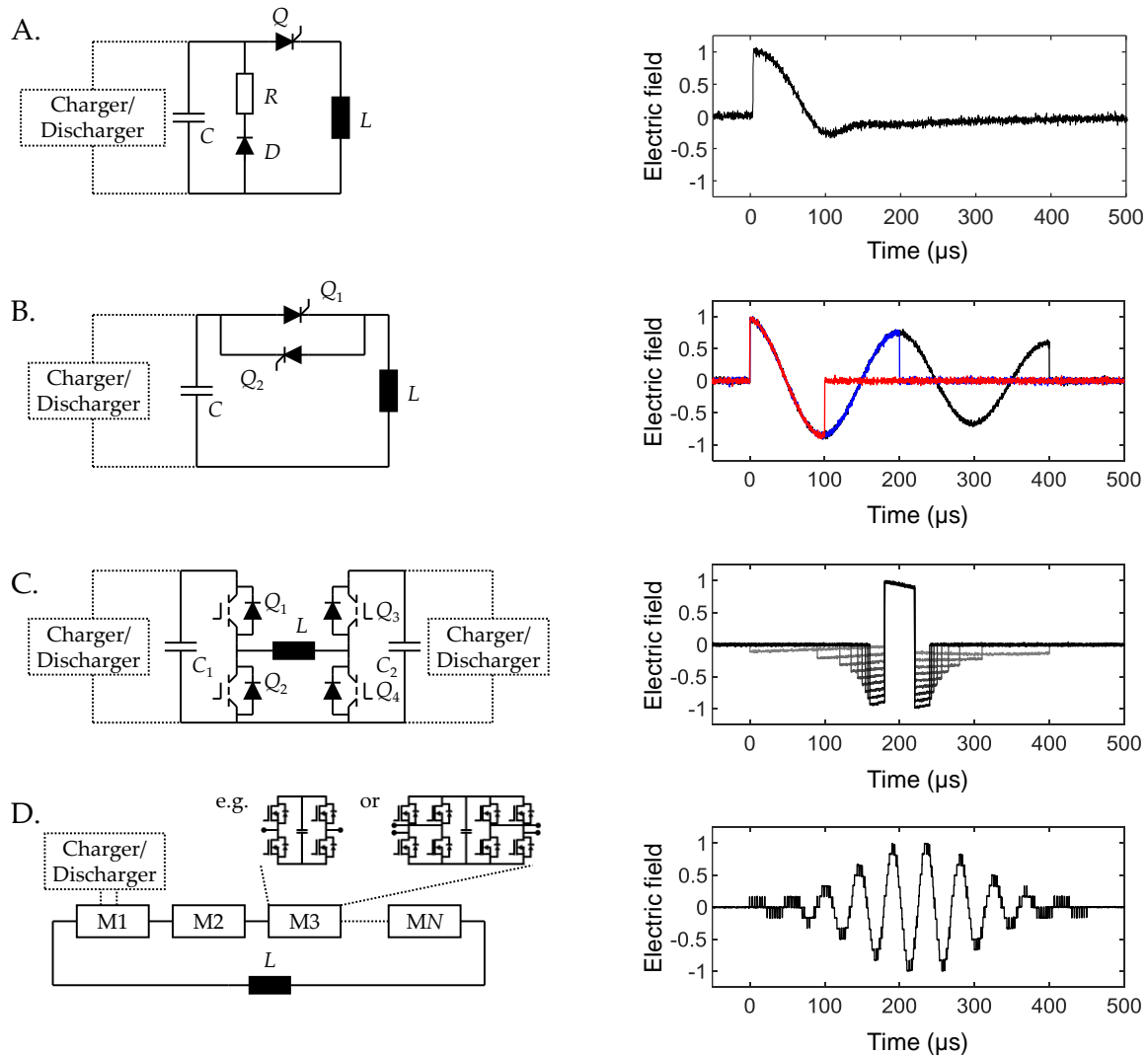
Figure 1. Circuit topologies (left column) and corresponding typical pulse shapes (right column) of various TMS technologies: A. Monophasic stimulator (typically with thyristors), B. bi- and polyphasic stimulator (existing with thyristors and IGBTs), C. example of a bridge-based TMS device using IGBTs, representing also all other bridge approaches, and D. modular pulse synthesizer. This work implements six four-bridge modules (double H bridge) as shown on the right, which the control can intrinsically operate also as two-bridge modules (H bridge, shown as alternative on the left and compared in Table I). The topology can use chargers and dischargers in several positions. Although every module could have its own charger, a single one in combination with the circuit’s charge distribution capabilities is sufficient and can reduce common-mode currents through the parasitic and filter capacitances of the chargers, which are relevant for electromagnetic interference.
