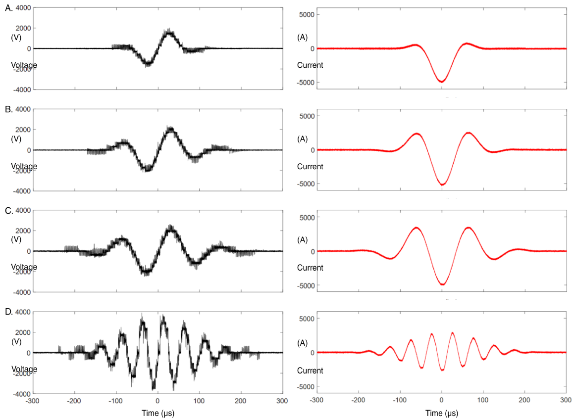
Figure 17. Polyphasic pulses with sinusoidal current and Gaussian envelope of increasing width from A to D. For very short envelope width, the pulse degenerates into a near-sinusoidal biphasic pulse, which in contrast to conventional biphasic TMS pulses contains smoother edges in the voltage.
