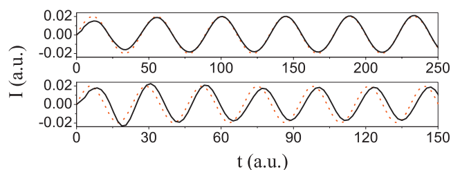
FIG. 9. Current as a function of time for H_2 molecules subjected to ac signals of two frequencies, as in Figs. 7(c) and 7(d). A larger extended molecule is used: six atoms on each side of the molecule in contrast to four in Fig. 7. A well-coupled case (solid, d_1=1.5 \text{ \AA} ) is compared to the applied voltage (dotted, 1 V amplitude); the interatomic distance in the leads is 1.5 \text{ \AA} .
