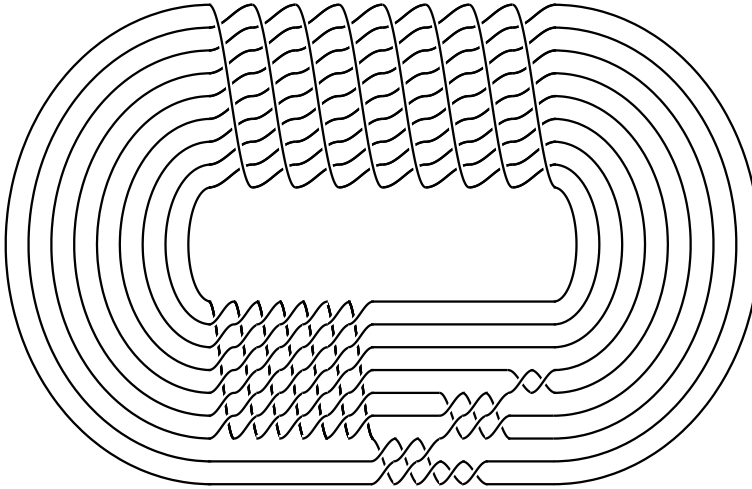
FIGURE 3. A topologically slice knot obtained as the closure of the braid word
