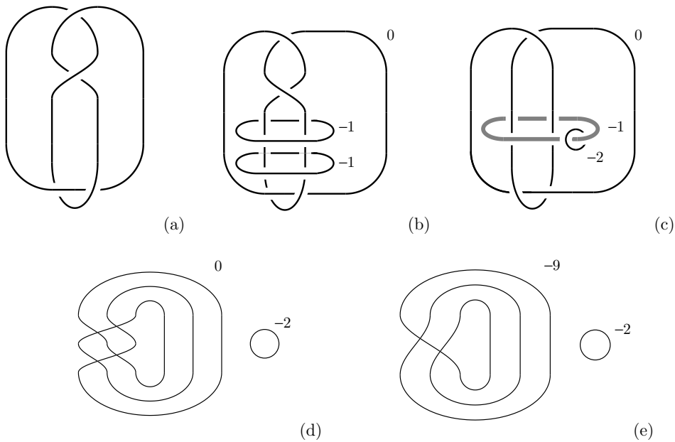
FIGURE 1. A sequence of blow up and blow downs showing that S_0^3(4_1) bounds a spin manifold with b_2 = 11 and \sigma = 8 . The characteristic link at each stage is specified by darker curves.
