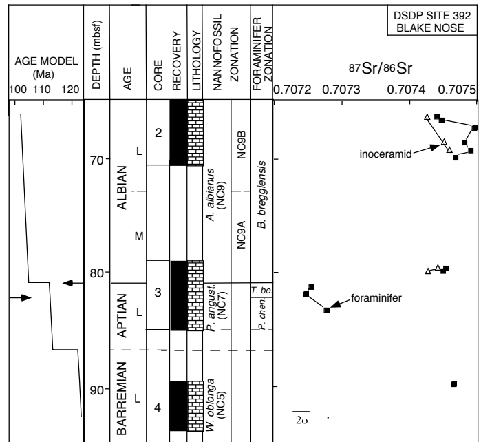
Figure 12. Strontium-isotope data from Hole 392A. The nanofossil biostratigraphy is after Schmidt (1979), modified as part of this study. Planktic foraminiferal biostratigraphy is modified after Gradstein (1978). An age model is shown on the left; arrows signify tie points (see Table 2). The key to the lithologic column is given in Figure 5; mbsf—meters below sea floor.
