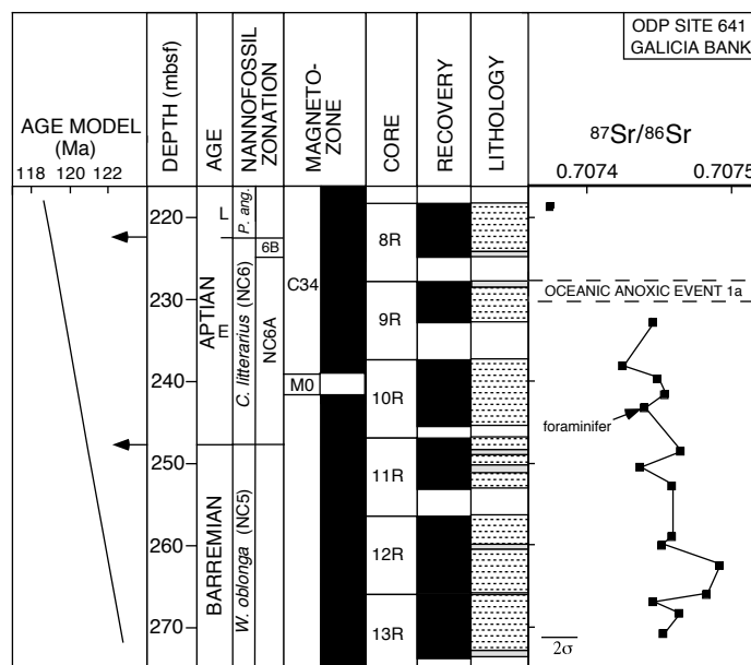
Figure 16. Strontium-isotope analyses of foraminifers from Hole 641C. The nannofossil biostratigraphy is after Applegate and Bergen (1989), modified by Bralower et al. (1994). An age model is shown on the left; arrows signify tie points (see Table 2). Position of oceanic anoxic event OAE1a of Bralower et al. (1993) is shown. The key to the lithologic column is given in Figure 5; mbsf—meters below sea floor.
