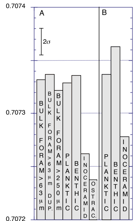
Figure 3. Comparison of 87 Sr/ 86 Sr values of different fossil components in samples from Site 511. (A) Sample 511-56-3, 43–45 cm. (B) Sample 511-55-3, 39–41 cm. Bulk foram.—combined benthics and planktics; Dup.—duplicate analysis; Ostrac.—ostracods.
