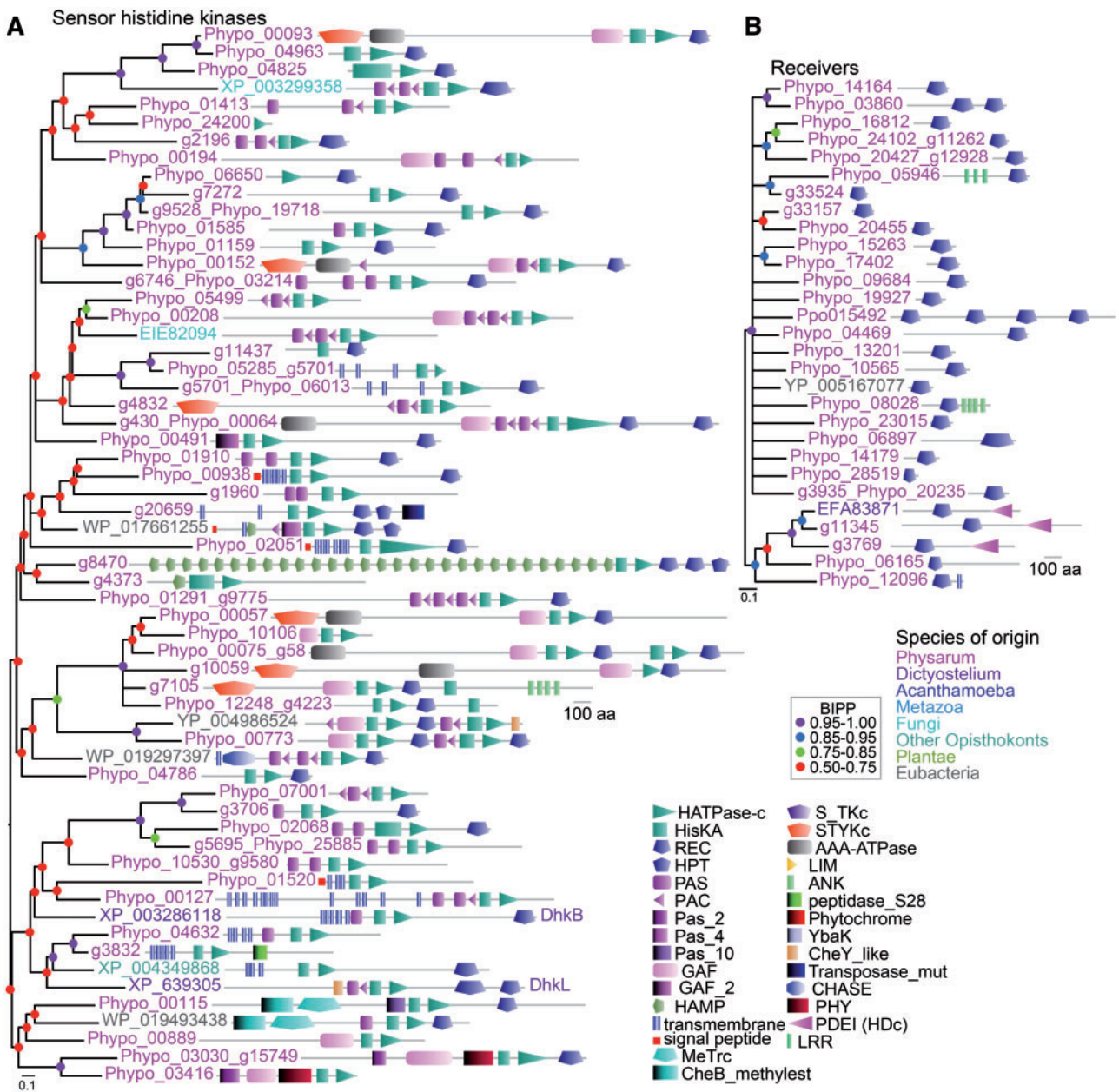
FIG. 4. —Sensor histidine kinases/phosphatases and phosphorelay receivers. (A) Sensor histidine kinases/phosphatase . The P. polycephalum genome was queried by BLAST with all 15 Dictyostelid SHKPs, plant and fungal SHKPs, and the most divergent prokaryote SHKPs, while transcribed proteins were queried for the presence of Interpro domains IPR003661 and IPR003594 for the HisKA and HATPase-c moieties of SHKPs, respectively. The retrieved sets largely overlapped, but the transcriptome (Phydo identifiers in the tree) contained both the largest number and more complete SHKPs. Sequences were first aligned with all their closest relatives in other organisms, as identified by BlastP of the GenBank non-redundant sequences. However, in a phylogeny constructed from this alignment, most of the outgroup sequences clustered together. Their contribution therefore was reduced to the ones with greatest identity to individual clusters of P. polycephalum SHKPs. A second phylogeny was constructed from these outgroup and P. polycephalum sequences, using only segments encompassing the HisKA, HATPase-c, and receiver domains, which are common to all or most retrieved SHKPs. The tree was annotated with the functional domain architecture of the proteins. The methods used for sequence alignment, alignment editing, and Bayesian phylogenetic inference are the same as described in the legend to supplementary fig S13 . Protein tags are color-coded to reflect the species of origin as shown, and Bayesian posterior probabilities of tree nodes are represented by colored dots. (B) Receivers . Putative effectors for SHKP activated signaling were identified by query of genome and transcriptome sequences with receiver/response regulator protein sequences or the Interpro identifier IPR001789 for this domain, respectively, leaving out all proteins that also contained HisKA or HATPase-c domains. Query for outgroup sequences mainly retrieved SHKPs, which also contain a receiver domain, and Dictyostelium RegA. RegA and one other none-SHKP outgroup sequence (YP_005167077) were aligned with the P. polycephalum sequences, and a phylogenetic tree was constructed by Bayesian inference as described above. The tree was decorated with protein domain architectures.
