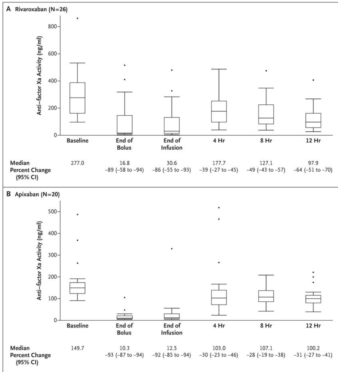
Figure 1. Anti-Factor Xa Activity and Percent Change from Baseline in Patients Receiving Rivaroxaban and Apixaban (Efficacy Population)
