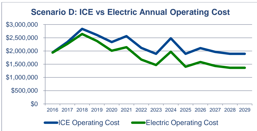
Figure 16. Scenario D: Comparison of Annual Operating Costs, ICE vs. Electric
