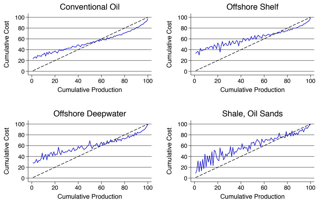
Figure 8. : Costs over the Field Lifecycle
