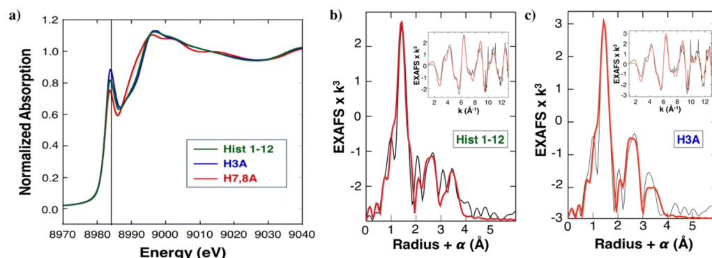
Figure 5. X-ray absorption spectroscopy data for Hist 1–12, H3A, and H7,8A. (a) XANES spectra of Hist 1–12 (green), H3A (blue), and H7,8A (red). The vertical line is 8984 eV. EXAFS spectra of (b) Hist 1–12 and (c) H3A ( k^3 -weighted) in k space ( \text{\AA}^{-1} ) and the corresponding Fourier transform of the data ( \text{\AA} , offset by phase shift \alpha ). Unfiltered and unsmoothed data are shown as the thin line in each frame; the thick line represents the best five- and four-shell fit to the data (for Hist 1–12 and H3A, respectively, as shown in bold in Table S1). Data were fit over a k range of 1\text{--}13 \text{\AA}^{-1} .
