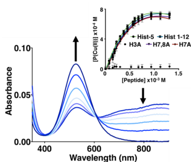
Figure 3. Cu(II)-binding competition with NTA as a competitive chelator. Optical titration of \leq 2 equiv of Hist-5 into a 0.8 mM NTA/Cu(II) solution (1:1) in 50 mM HEPES buffer (pH 7.4). The inset shows a comparison of titration data from all peptides, showing the increase of the Cu–peptide complex (taken from the \text{Abs}_{850} decrease) as a function of added peptide. All of the peptides compete effectively with NTA for Cu(II), with the exception of H3A, the only sequence lacking an ATCUN motif. Lines represent the best fit to eq 2, and error bars represent the standard deviation from the average of triplicate measurements.
