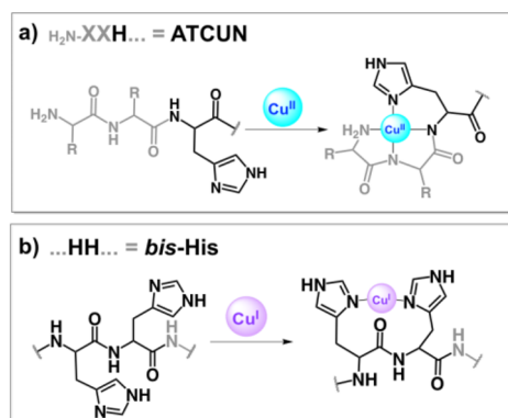
Figure 1. Signature Cu-binding motifs present in histatin peptides. (a) A free amino terminus and a histidine in the third position make ATCUN motifs (amino-terminal Cu/Ni binder) favorable for square planar Cu(II). (b) Adjacent histidines (bis-His) anchor Cu(I) in a linear fashion but can accommodate higher coordination if additional ligands contribute (only linear shown).
