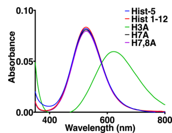
Figure 2. Absorption spectra of Cu(II)-bound peptides. Absorption spectra of Hist-5 and model peptides (1 mM) with 0.8 equiv of CuSO 4 in 50 mM HEPES buffer (pH 7.4). The absorbance feature at 530 nm (ε = 110 M −1 cm −1 ) is characteristic of a Cu(II)-bound ATCUN site. Replacement of the third His abolishes the ATCUN site, hence the red-shift of the absorbance to ~620 nm for peptide H3A.
