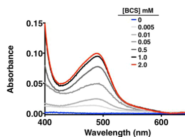
Figure 7. Cu chelator BCS is capable of outcompeting Hist-5 for Cu binding. UV-vis spectra of 7.0 μM Hist-5 and 7.0 μM Cu(II)SO 4 in YPD medium incubated for 1 h with a BCS concentration increasing from 0 to 2 mM.
