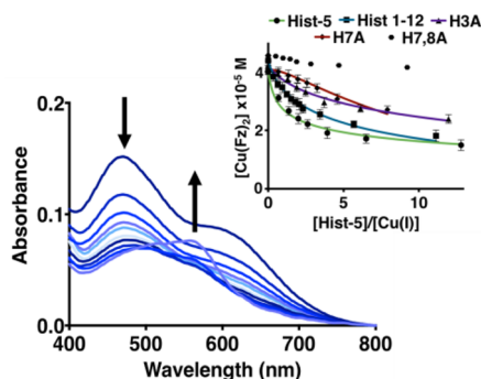
Figure 4. Cu(I)-binding competition using Fz as a competitive chelator. Optical titration of Hist-5 to a 55 \mu\text{M} solution of [\text{Cu(I)}(\text{Fz})_2]^{3-} in 50 mM HEPES buffer (pH 7.4) under anaerobic conditions. The inset shows a comparison of the ability of all the peptides to outcompete Fz for Cu(I) binding. Error bars represent the standard deviation from the average of triplicate measurements; lines represent the best fit to the equilibrium expressed in eqs 7 and 8 (see the Experimental Section).
