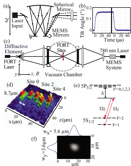
FIG. 1. (Color online) (a) MEMS steering system schematic. (b) Mirror tilt transient response when voltage is applied (left) or removed (right) at time t=0 . (c) Schematic of the experimental setup showing the FORT beams and the 780 nm ground state Rabi laser. (d) Averaged fluorescence image of the five trap sites over many trap loading periods. Each site is separated by 8.7 \mu\text{m} . (e) Energy level structure showing the two photon Raman transition used for single qubit rotations. (f) Image and profile of the focused ground state Rabi laser at the atom.
