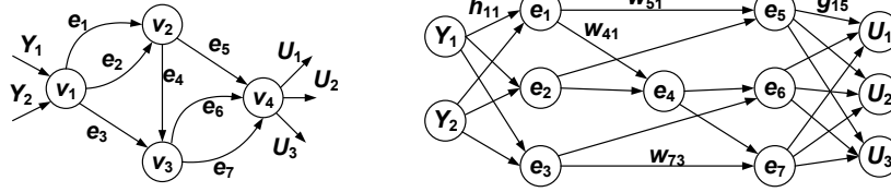
Fig. 4. (a) Point to point communication in a simple network [12]; Sources \mathbf{Y}_{1:2} represent input processes, \mathbf{U}_{1:3} denotes the network outputs; (b) The directed labeled line graph for the graph from (a) (only some of the links have been labeled to reduce clutter).
