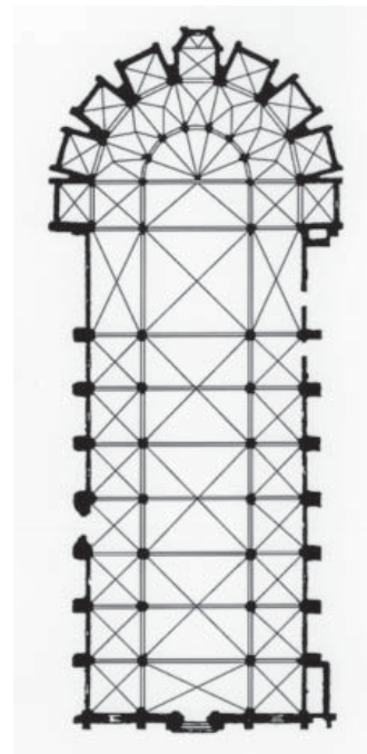
13. Bologna, San Francesco: a. in 1766 [RULLO, 2012, fig. 7]; b. after nineteenth-century restorations [SCHENKLUHN, 2000, p. 70].
