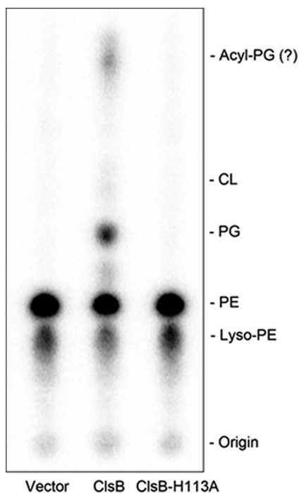
FIGURE 5. In vitro conversion of PE to PG by ClsB . [ ^{32} P]PG was formed by mixing membranes derived from BKT29 cells expressing wild-type ClsB and partially purified ^{32} P-labeled PE in the presence of 100 mM glycerol. In contrast, no PG was formed using membranes from cells transformed with an empty vector or expressing the ClsB H113A mutant. The presence of ^{32} P-labeled lyso-PE likely resulted from partial hydrolysis of PE. The spot at the top of the second lane concurrent with PG formation is likely acyl-PG, a known PG derivative in E. coli .
