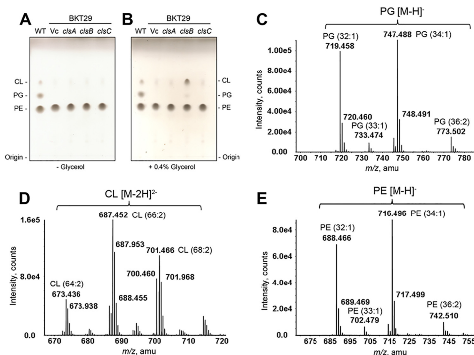
FIGURE 3. Synthesis of PG and CL by ClsB in the \Delta pgsA \Delta clsABC (BKT29) mutant cells expressing ClsA, ClsB, or ClsC. The trace spot detected near CL in the vector control sample was previously identified by LC/MS/MS to be undecaprenyl-phosphate ( C_{55} -P) (2). B, the addition of glycerol to the growth medium greatly increased the production of PG and CL by ClsB (to near wild-type levels). C and D, MS analysis of PG and CL produced as a result of ClsB expression and glycerol supplementation in BKT29. PG (C) and CL (D) were detected by LC/ESI/MS in the negative ion mode primarily as singly charged [M-H]^- and doubly charged [M-2H]^{2-} ions, respectively. The acyl compositions of PG species are almost identical to those of PE (E), hinting the phosphatidyl groups of PG were transferred from PE species.
