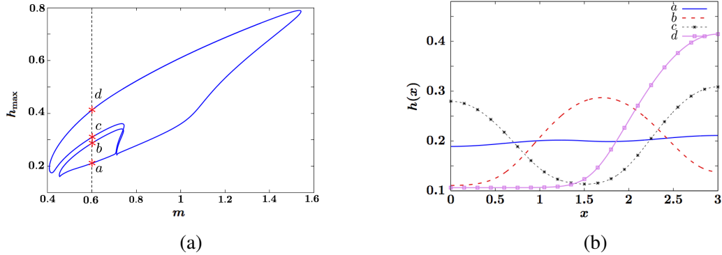
FIG. 20: (a) Part of the bifurcation diagram from Fig. 3(c) highlighting four distinct non-primary steady-states with mass m = 0.6 . (b) The corresponding height profiles of the four solutions, of which a - c were shown in Fig. 3(e) and d is a large droplet centered at x = L .
