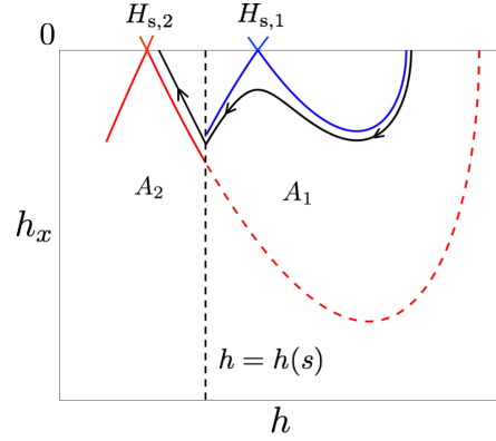
FIG. 15: Schematic phase plane diagram showing the homoclinic orbits for A(x) \equiv A_1 (blue) and A(x) \equiv A_2 (red) and the trajectory for a branch 2 solution.
