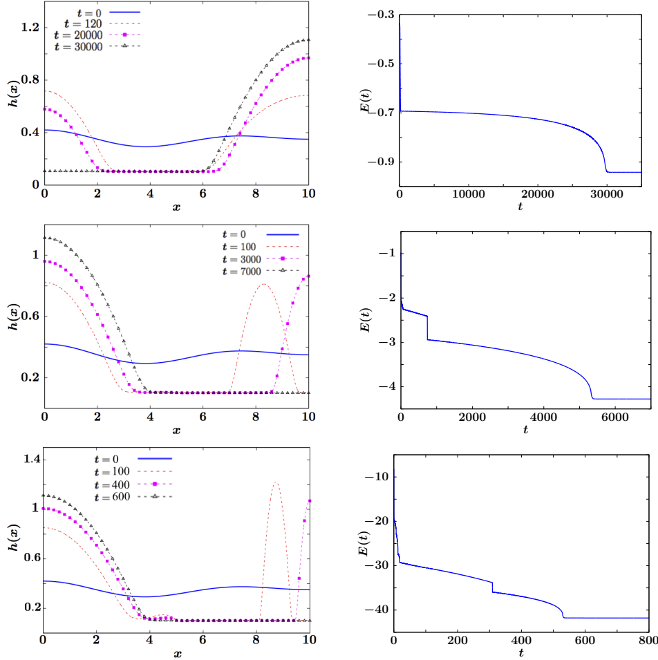
FIG. 22: Dewetting dynamics of thin films over time starting from the same initial profile on 0 \leq x \leq 10 with \varepsilon = 0.1 . Each row shows height profiles h(x, t) at selected times (left) and the evolution of the energy (2.6) (right). (Top) Evolution on a homogeneous substrate, A(x) \equiv 1 , (Middle) evolution on a heterogeneous substrate with A_2 = 5 on 5 \leq x \leq 10 , (Bottom) evolution on a heterogeneous substrate with A_2 = 50 on 5 \leq x \leq 10 . Note the differences in time-scales and the differences in the final states of the solutions.
