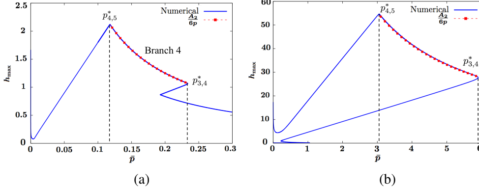
FIG. 9: Bifurcation diagram \bar{p} vs. h_{\max} computed numerically and compared with the asymptotic prediction of branch 4 (a) in the limit \varepsilon \rightarrow 0 , with parameters A_1 = 1 , A_2 = 1.5 , \varepsilon = 0.001 . (b) in the limit A_2 \rightarrow \infty , with parameters A_1 = 1 , A_2 = 1000 , \varepsilon = 0.1 . In both (a) and (b), L = 6 , s = 3 . The blue solid curve represents the numerically computed bifurcation curve. The red dashed and dotted curve represents the asymptotic prediction given by (3.9).
