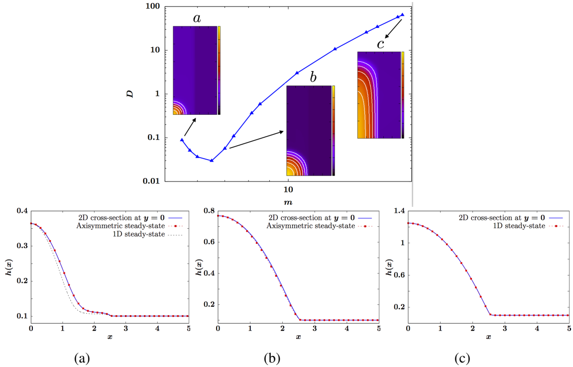
FIG. 24: Thin films on a hydrophilic stripe, -s \leq x \leq s : (top) Film mass m vs. D plotted in log scale for both droplet-type solutions and perturbations of thick flat films, with parameters L_x = 5 , L_y = 10 , A_1 = 1 , A_2 = 10 , s = L_x/2 . The insets show color contour maps of three selected solutions (on one quarter of the domain, reduced by symmetry). (a,b,c) Cross-section of the two-dimensional solutions at y = 0 compared with the axisymmetric and one-dimensional steady-states with the same maximum film thickness for droplets a, b, c respectively.
