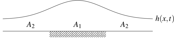
FIG. 1: Schematic diagram of a thin film on a heterogeneous substrates with stepwise chemical patterning yielding relatively hydrophilic ( A_1 ) and hydrophobic ( A_2 > A_1 ) regions.
