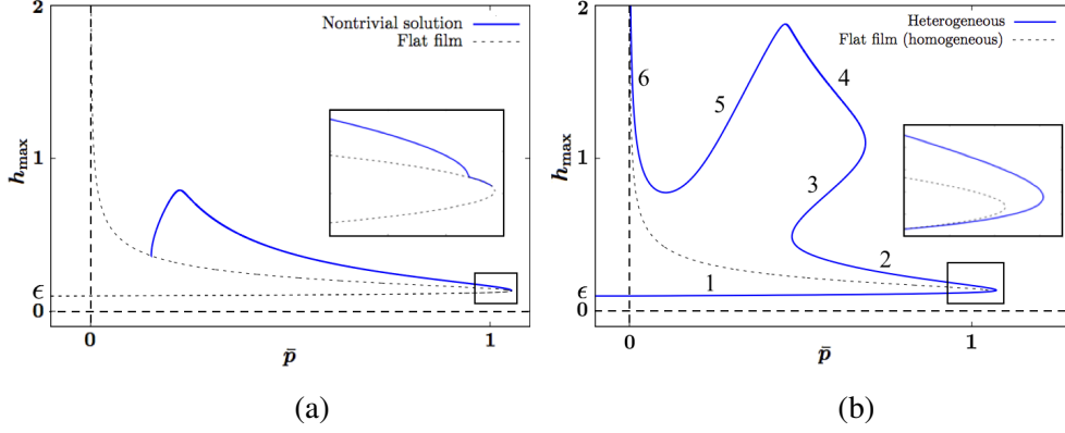
FIG. 4: Bifurcation diagram of \bar{p} vs. h_{\max} for steady-states with \varepsilon = 0.1 and L = 3 on (a) a homogeneous substrate A(x) \equiv 1 . (b) on a heterogeneous substrate with A_1 = 1, A_2 = 5, s = 1.5 . The solid blue curve represents nontrivial steady-state solutions. The dashed black curve in (a) represents two branches of flat film solutions that merge together with the nontrivial branch at \bar{p} = p_{\max} . In both (a) and (b), the inset plot shows the bifurcation curve zoomed into a small neighborhood near the maximum pressure.
