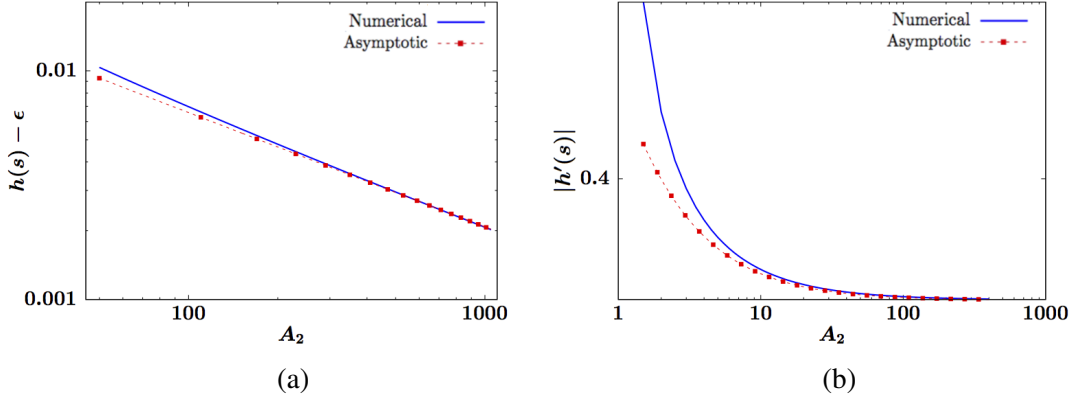
FIG. 12: Properties of branch 3 pinned droplet solutions computed with parameter values A_1 = 1, L = 6, s = 3, \varepsilon = 0.1 : (a) Comparison of h(s) - \varepsilon computed numerically with \bar{p} = 0.292 (blue) and from the asymptotic approximation (3.31) (red dots) for large A_2 plotted on log scale. (b) the contact angle |h'(s)| vs. A_2 with fixed pressure \bar{p} = 0.22 , plotted on log scale, the numerical result (blue) compared with the asymptotic prediction (3.33) (red dots).
