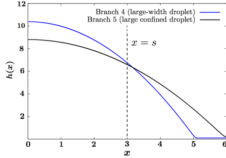
FIG. 7: Profiles of two droplet solutions with mass m = 35.2 on the domain L = 6 for a disjoining pressure with A_1 = 1 , A_2 = 50 , L = 6 , s = 3 , \varepsilon = 0.1 . A typical branch 4 large-width droplet, with s < w < L , is shown by the blue curve for \bar{p} = 0.493 and a branch 5 confined droplet, with w = L , at pressure \bar{p} = 0.809 is given by the black curve.
