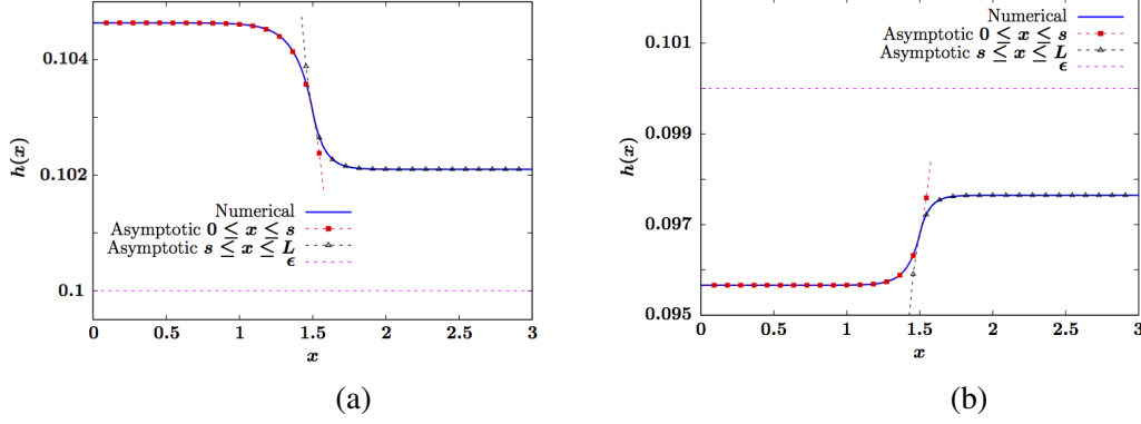
FIG. 5: Properties of branch 1, small-thickness film solutions, computed with parameters A_1 = 1 , A_2 = 2 , s = 1.5 , \varepsilon = 0.1 : (a) A numerical solution (blue) with \bar{h} > \varepsilon compared with approximate form (3.3) (dotted curves). (b) A computed solution (blue) with \bar{h} < \varepsilon also compared with (3.3).
