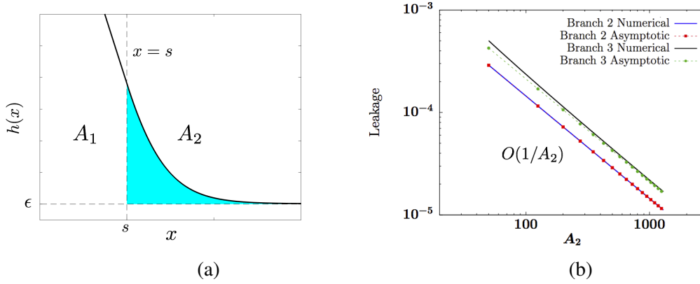
FIG. 16: (a) Schematic illustration of fluid leakage (4.2) (b) Leakage as a function of A_2 computed numerically and asymptotically for a branch 2 solution with \bar{p} = 0.466 and a branch 3 solution with \bar{p} = 0.38 plotted in log scale. The asymptotic prediction for branch 2 and branch 3 is given by (4.4) and (4.5) respectively. The pressure \bar{p} is fixed as A_2 increases with L = 6 , s = 3 , A_1 = 1 , \epsilon = 0.1 .
