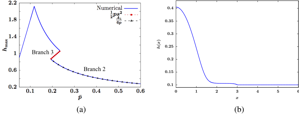
FIG. 13: Properties of small and pinned droplets: (a) The bifurcation diagram for \bar{p} vs. h_{\max} highlighting branches 2 and 3. The solid blue curve gives numerical results. The black and red dotted curves represent the asymptotic prediction of h_{\max} for branch 2 and branch 3 solutions respectively in the limit \varepsilon \rightarrow 0 , with parameters A_1 = 1 , A_2 = 1.5 , L = 6 , s = 3 , \varepsilon = 0.001 . (b) Profile of a steady-state on branch 2, characterized by a droplet on [0, s] and nearly-uniform thin film on [s, L] .
