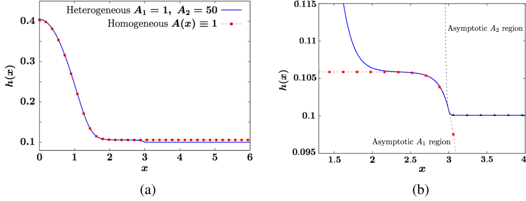
FIG. 14: Details for a branch 2 solution computed with parameters L = 6 , s = 3 , A_1 = 1 , A_2 = 50 , \varepsilon = 0.1 , \bar{p} = 0.467 : (a) Comparison of the numerical solution (blue) on the heterogeneous substrate with its corresponding A_1 -homogeneous homoclinic (red dots) with the same pressure. (b) Comparison of the numerically computed steady-state (blue) and the approximations (3.35, 3.29) for the structure near the interface x = s (red, black dots).
