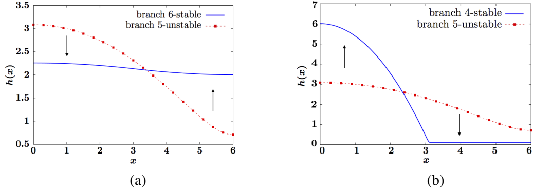
FIG. 18: Bi-stable dynamics with respect to perturbations of an unstable branch 5 solution h_*(x) . (a) Initial conditions (red dotted curve) h(x, 0) = h_*(x) + \delta g_1(x) , with g_1(x) being the unstable eigenmode of h_* and small \delta > 0 , evolving to the stable branch 6 solution (blue curve). (b) Initial conditions h(x, 0) = h_*(x) - \delta g_1(x) evolving to the stable branch 4 solution.
