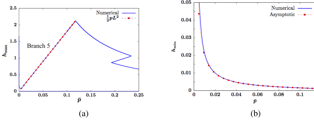
FIG. 10: Properties of branch 5 large drop solutions computed with parameter values A_1, A_2 = 1.5 , L = 6 , s = 3 , \varepsilon = 0.001 : (a) Branch 5 highlighted in the bifurcation diagram for \bar{p} vs. h_{\max} computed numerically (blue solid curve) and compared with the asymptotic estimate (3.15) (red dotted curve) in the limit of small \varepsilon . (b) The minimum, h_{\min} as a function of \bar{p} computed numerically (blue solid curve) and the asymptotic result (3.17, 3.18) (red dotted curve).
