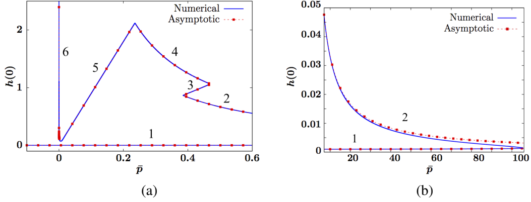
FIG. 17: Bifurcation diagram for h(0) = h_{\max} vs. p for (a) small p . (b) large p . The solid curve denotes the numerically computed bifurcation curve. The dashed and dotted curve denotes the asymptotic prediction of h_{\max} derived for each branch in the limit of small \varepsilon . In both (a) and (b), A_1 = 1 , A_2 = 1.5 , L = 6 , s = 3 , \varepsilon = 0.001 .
