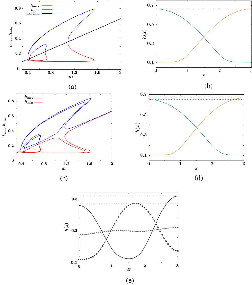
FIG. 3: Steady solutions with \varepsilon = 0.1 on a domain of length L = 3 : (a) Bifurcation diagram of m vs. h_{\min}, h_{\max} for solutions on homogeneous substrate, A(x) \equiv 1 . (b) Profile of two steady-state droplets from (a) with m = 1.1 centered at x = 0 and x = L . (c) Bifurcation diagram of m vs. h_{\min}, h_{\max} for steady-state solutions on stepwise-patterned substrate with A_1 = 1 , A_2 = 1.1 and s = L/2 . (d) Asymmetric steady-state droplets centered at x = 0 and x = L both with mass m = 1.1 . The difference in the maximum film thicknesses is highlighted by the two dashed lines. (e) Profiles of three distinct inner loop steady-state solutions on stepwise-patterned substrate, all with mass m = 0.6 .
