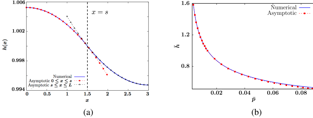
FIG. 6: Properties of branch 6, thick film solutions, computed for parameters \varepsilon = 0.1 , A_1 = 1 , A_2 = 2 , L = 3 , s = 1.5 : (a) A numerically computed solution (blue) compared with the asymptotic estimates (3.5) (dotted) at pressure \bar{p} = 0.0135 . (b) The computed mean thickness \bar{h} (blue) as a function of \bar{p} compared with the asymptotic prediction (3.7) (red dots).
