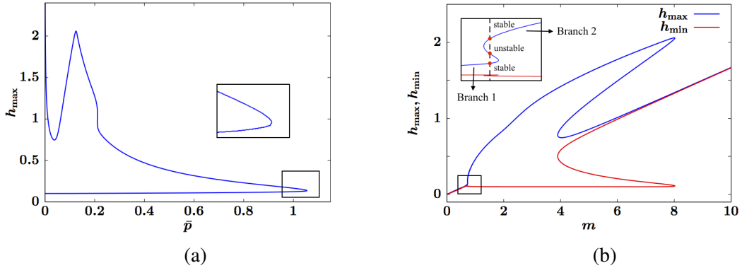
FIG. 19: Bifurcation diagrams for parameters L = 6 , s = 3 , A_1 = 1 , A_2 = 1.5 , \varepsilon = 0.1 : (a) bifurcation diagram for \bar{p} vs. h_{\max} (b) bifurcation diagram for m vs. h_{\max}, h_{\min}
