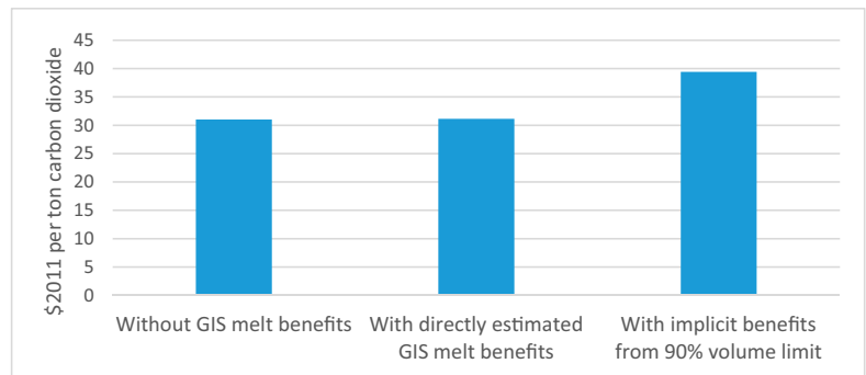
Fig. 1. Estimated 2015 social cost of carbon with and without GIS melt benefits. Data from table 2 and SI appendix, table J-2 of ref. 4.
