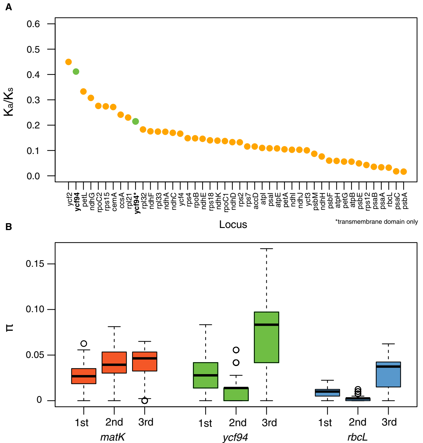
FIGURE 2. Comparison of ycf94 with other plastid genes. (A) K_a/K_s values of 49 loci across 20 fern plastomes plotted in descending order. The values for ycf94 are highlighted in green for both the entire ORF and the putative transmembrane domain (asterisk). (B) Sequence variation at the first, second, and third codon positions for Deparia matK , ycf94 , and rbcL .
