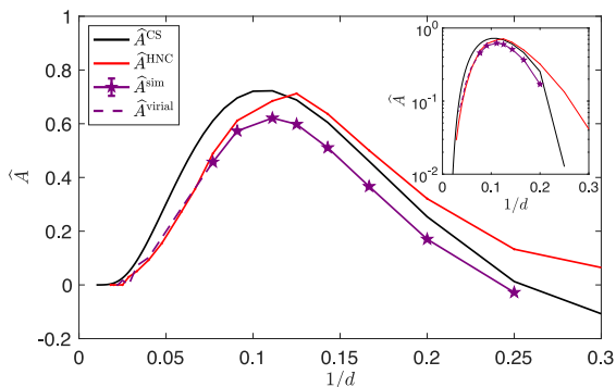
Figure 3. Fitting coefficients for the CS form, \hat{A}^{\text{sim}} (purple stars), grow from a negative value for d < 5 to a peak in d = 9 , before steadily decreasing. This behavior is consistent with prediction for \hat{A}^{\text{CS}} [31] (black), to which the numerical results could plausibly converge at even higher d than is reached here. The quantity should therefore vanish as d \rightarrow \infty . The dimensional range is extended by fitting the virial (purple) and HNC (red) [32] up to d = 50 to a CS form. High- d convergence is best assessed on a logarithmic scale (inset).
