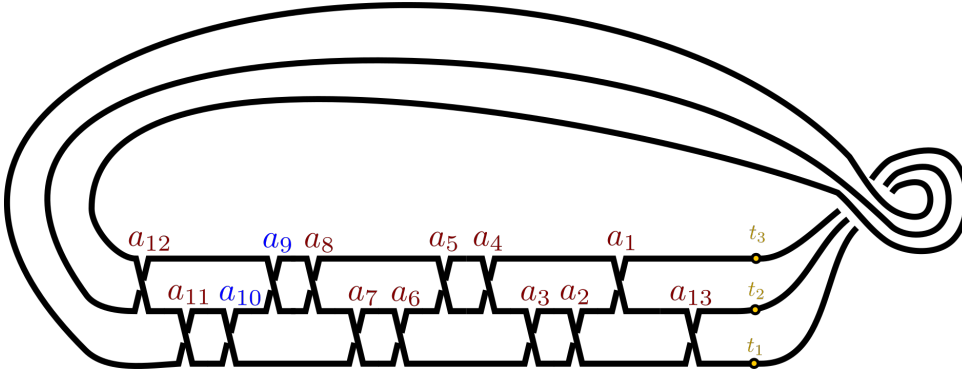
FIGURE 30. Lagrangian projection for the Legendrian link \Lambda_1 , as used in the proof of Theorem 6.4. In this proof, the crossings a_{10}, a_9 , in blue, are used to detect the infinite order of the \vartheta -monodromy. The \vartheta -monodromy is obtained by moving the purple box around this projection. To construct \Lambda_2 instead, add an additional crossing labeled a_{14} to the purple box, between a_{13} and the base points t_1, t_2 .
