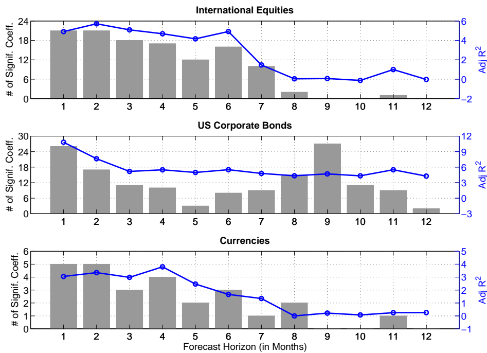
Figure 2 B: This figure shows the average adjusted R 2 (line, right y-axis) and number of significant coefficients (bars, left y-axis) of the hedge fund illiquidity index for different forecast horizons (in months). The results are for multiple predictor in-sample regressions, i.e. the hedge fund illiquidity index is included together with competitor variables.
