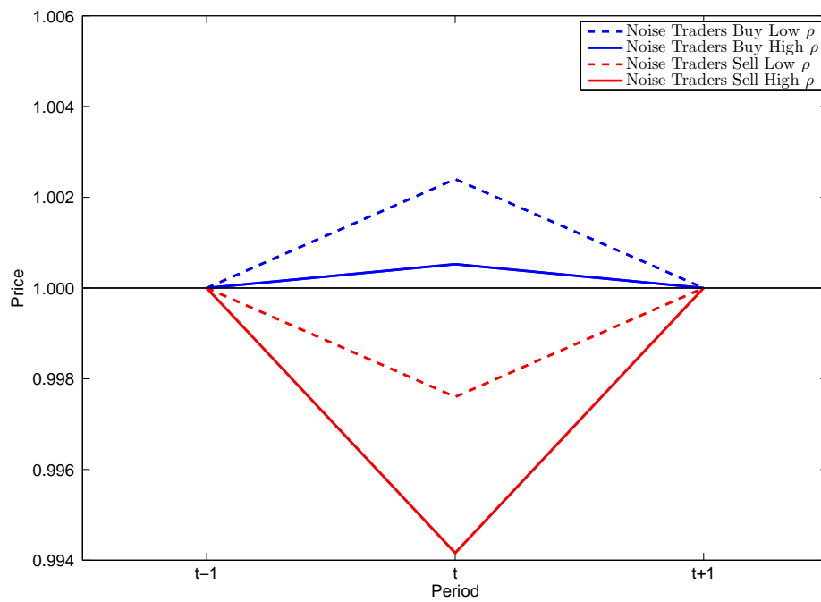
Figure Appendix A.1: This figure depicts the average return reversal implied by the model for the parameter values given in Table 5. The high \rho case corresponds to \theta = 8 and \lambda = 0.002 , and the low \rho case corresponds to the model without shortfall penalty, i.e. \lambda = 0 .
