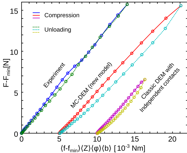
FIG. 6. (Color online) Validation that the scaling law from Ref. [8], derived from experimental data, also holds in the simulation. Here, F is the force exerted by the grains on the top plate, f is the average force at each contact, Z is the number of contacts per grain, \phi is the volume fraction within the packing (starting one diameter away from walls), and b is the distance between grain centers. Microscopic quantities were averaged on all grains and contacts within the packing. Data was then averaged on the 15 retained compression or unloading phases with the same strain. Each marker in the diagram represents one such strain level. MC-DEM and the usual DEM data have been shifted for clarity by 5 and 10 mNm, respectively.
