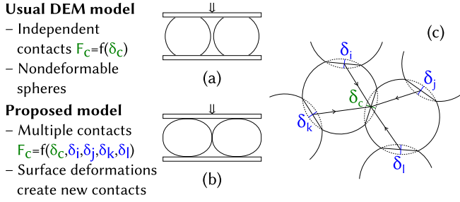
FIG. 1. (Color online) When squeezing a packing of particles, particles deform and new contacts are formed. Traditional DEM (a) does not take this into account. Our multiple contacts model (b) captures these by correcting contact deformation \delta_c using linearly additive corrections from other contacts \delta_{k \rightarrow c} , making (c) the local force depend on all particle contacts F_c = f(\delta_c, \delta_i, \delta_j, \delta_k, \delta_l) .
