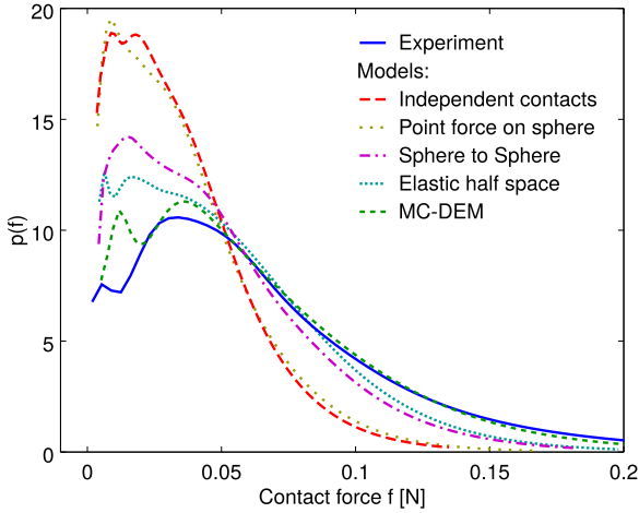
FIG. 4. (Color online) Comparison of the force distributions at intermediate compression \Delta = 18 mm during the unloading phase. This representative example is chosen to show values other than maximal compression. The bhat error measure in the main text captures all compression levels.
