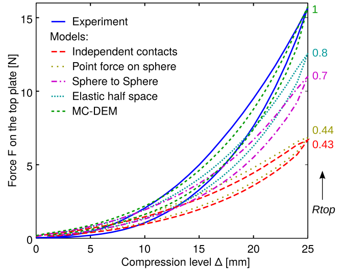
FIG. 3. (Color online) Force exerted on the top plate during a compression test, for the experimental data from [8] and all the simulation models mentioned above, for \mu = 0.03 .
