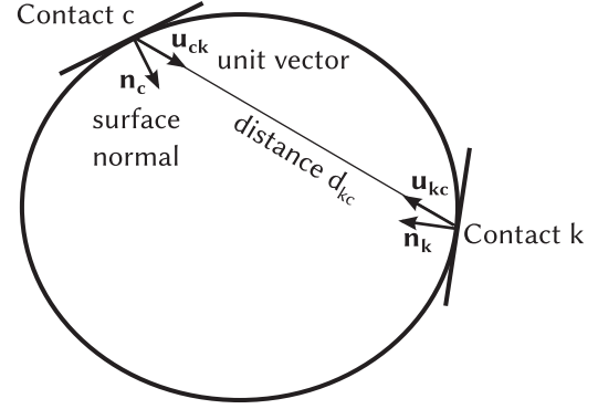
FIG. 2. Influence of one contact onto another. Contacts are not restricted to the surface of a sphere, their position is consistent with the grain deformations.
