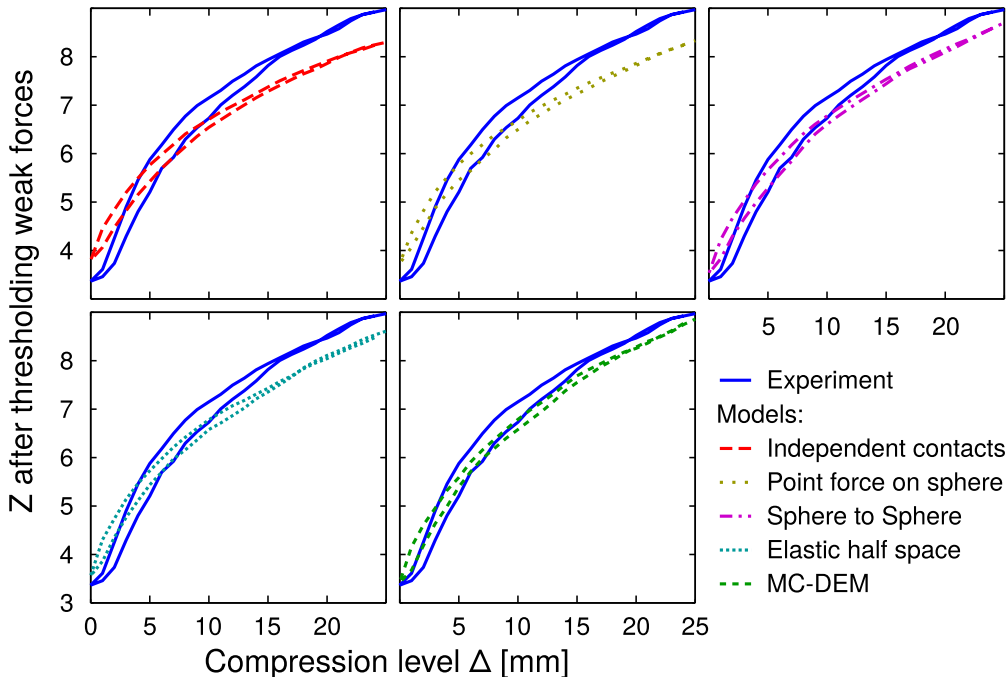
FIG. 5. (Color online) Number of contacts per grain Z after thresholding weak forces, averaged over multiple cycles.
