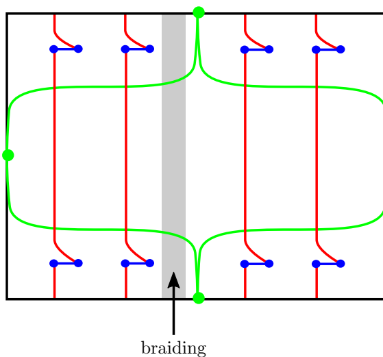
FIGURE 18. Additional short Reeb chords subdivide the Morse flow so that no points of equal height on the big disks are connected.
