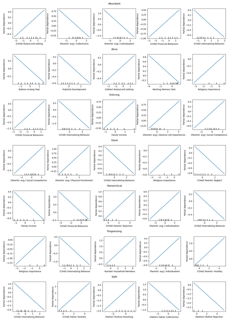
Figure 2: Partial dependence plots of the top five most important predictors for each Primal to show the direction of the effects between (normalized) predictor values and the outcome class. Positive slopes indicate that higher values of the predictor are associated with the “High” class; conversely, partial dependence plots with negative slopes indicate that higher values of the predictor are associated with the “Low” class.
