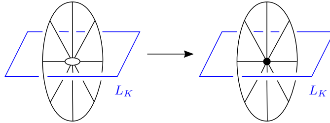
FIGURE 8. Elliptic boundary splitting.
