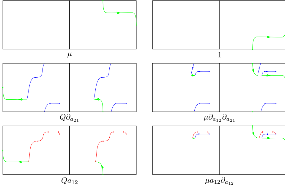
FIGURE 32. Geometry of coefficients for H(c_{22}) .
