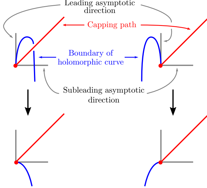
FIGURE 14. The crossings at a Reeb chord endpoint. The change or invariance of the real crossings are compensated by the change or invariance of imaginary crossings.
