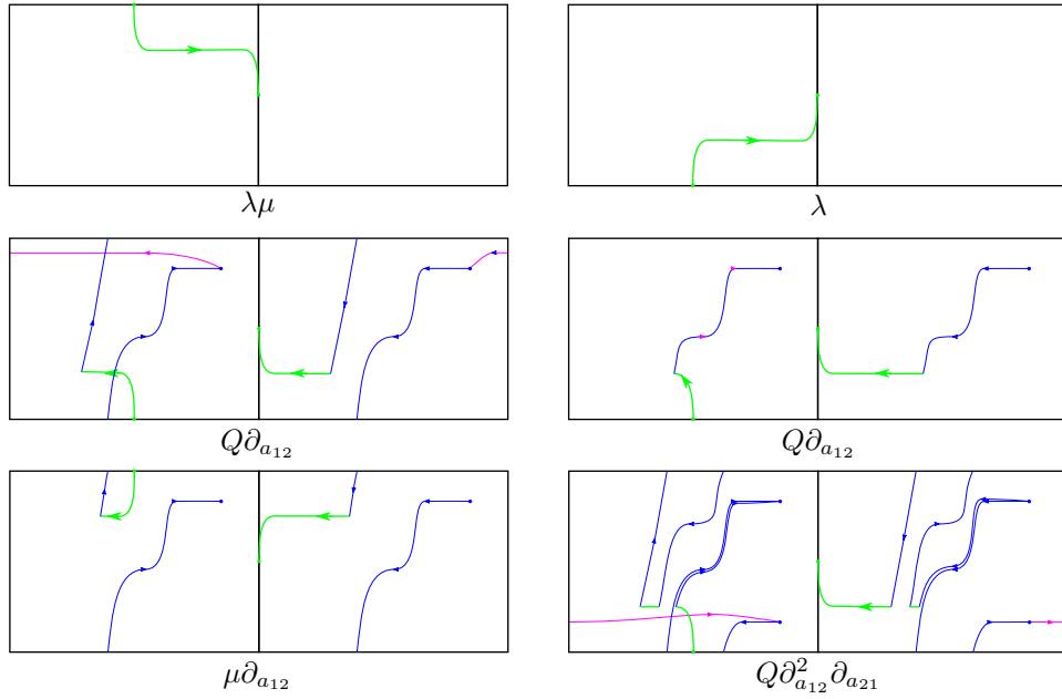
FIGURE 29. Geometry of coefficients for H(c_{11}) .
