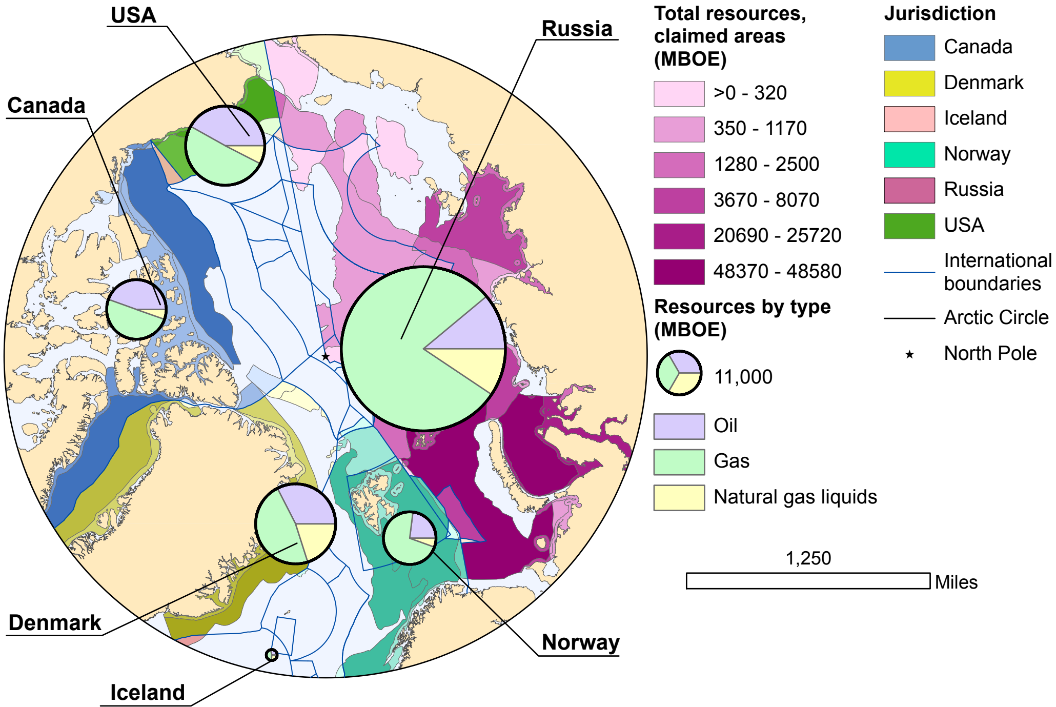
Map 2: Total Hydrocarbons in Undisputed and Claimed Areas
