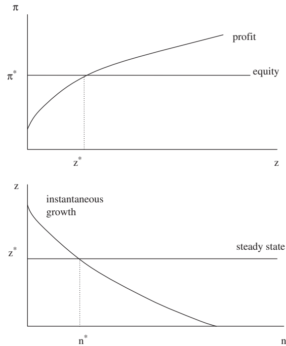
Fig. 3. Equilibrium with endogenous dividend tax rate.
