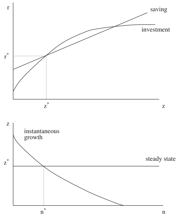
Fig. 2. Equilibrium with fixed tax rates.
