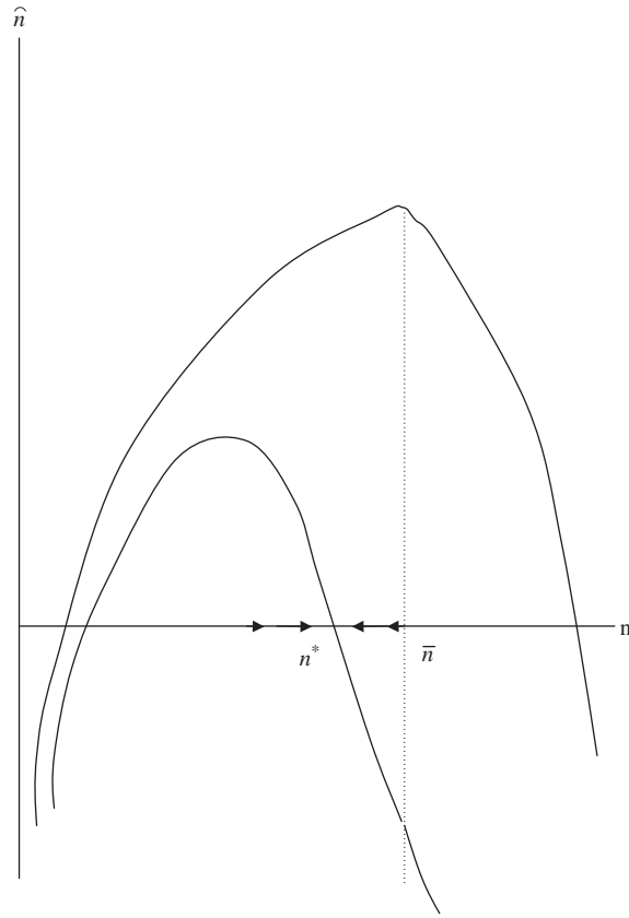
Fig. 1. Dynamics with fixed tax rates.
