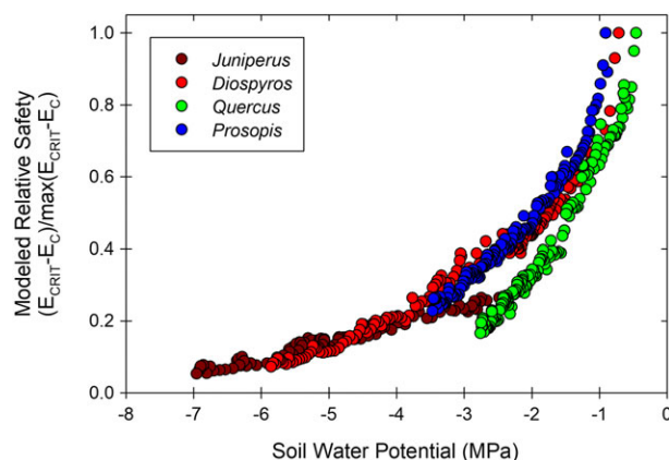
FIGURE 6 TREES simulated relative hydraulic safety as expressed as (E_{\text{CRIT}} - E_{\text{C}}) / \max(E_{\text{CRIT}} - E_{\text{C}}) versus the mean soil water potential experienced by the entire rooting volume for 2011
