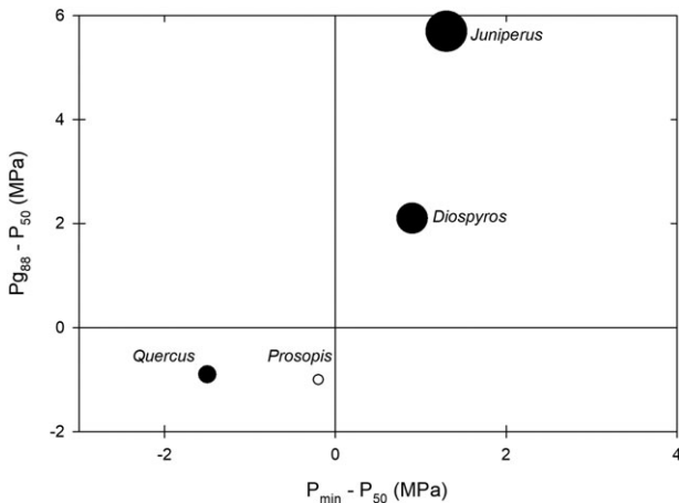
FIGURE 8 The degree of stomatal regulation of embolism ( P_{g88} - P_{50} ) versus hydraulic safety margin ( P_{min} - P_{50} ). Each symbol size is representative of the percent observed mortality for each species (with open symbol representing no mortality in Prosopis glandulosa )
