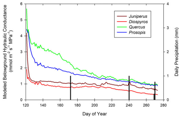
FIGURE 7 TREES simulated total belowground hydraulic conductance between May 1 and September 30, 2011. Vertical bars in Panel b represent daily precipitation in 2011
