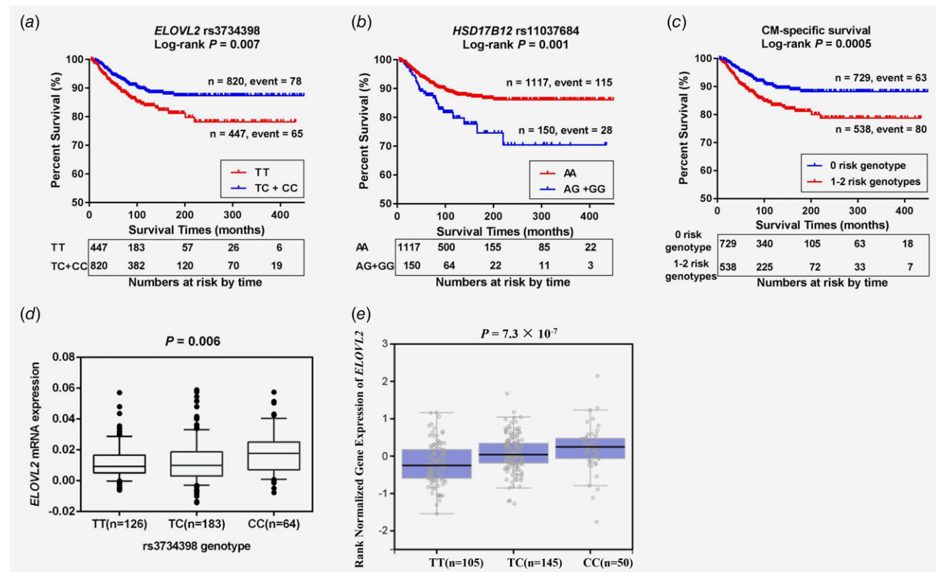
Figure 2. Two independent SNPs predict cutaneous melanoma survival and eQTL analysis for ELOVL2 rs3734398. Kaplan–Meier survival curves of CMSS stratified by ELOVL2 rs3734398 (a) and HSD17B12 rs11037684 (b), assuming a dominant model in the combined dataset of both MDACC and NHS/HPFS. (c) Kaplan–Meier survival curves of the combined risk genotypes on CMSS: dichotomized 0 risk genotype group and 1–2 risk genotypes group in the combined dataset of both MDACC and NHS/HPFS. The table below the Kaplan–Meier curves illustrates the numbers at risk for each time point. (d) The eQTL analysis for ELOVL2 rs3734398 in blood cells in the 1000 Genomes Project in an additive model. (e) The eQTL analysis from the Genotype-Tissue Expression project for ELOVL2 rs3734398 in an additive genetic model. Abbreviations: CM, cutaneous melanoma; CMSS, cutaneous melanoma-specific survival; ELOVL2 , elongation of very long-chain fatty acids 2; eQTL, expression quantitative trait loci; HSD17B12 , hydroxysteroid dehydrogenase type 12; MDACC, The University of Texas MD Anderson Cancer Center; NHS, the Nurses’ Health Study; HPFS, the Health Professionals Follow-up Study; SNP, single-nucleotide polymorphism.
