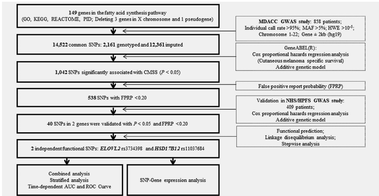
Figure 1. Study workflow for SNPs in the fatty acid synthesis pathway genes. Abbreviations: AUC, area under curve; CMSS, cutaneous melanoma-specific survival; ELOVL2 , elongation of very long-chain fatty acids 2; FPRP, false positive report probability; GWAS, genome wide association study; HSD17B12 , hydroxysteroid dehydrogenase type 12; HWE, Hardy Weinberg equilibrium; MAF, minor allele frequency; MDACC, The University of Texas MD Anderson Cancer Center; NHS, the Nurses' Health Study; HPFS, the Health Professionals Follow-up Study; ROC, receiver operating characteristic; SNP, single nucleotide polymorphism.
